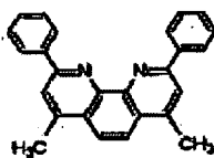
Structural formula 3:
